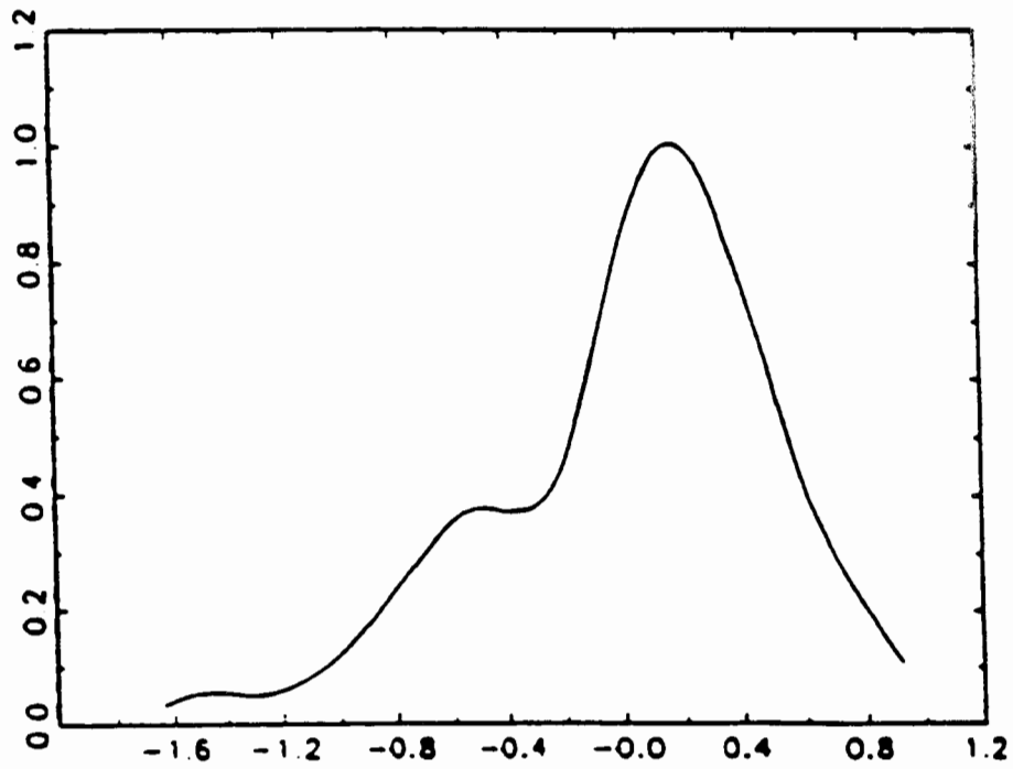
Figure 3.1 Single Index Function for Housing Data
