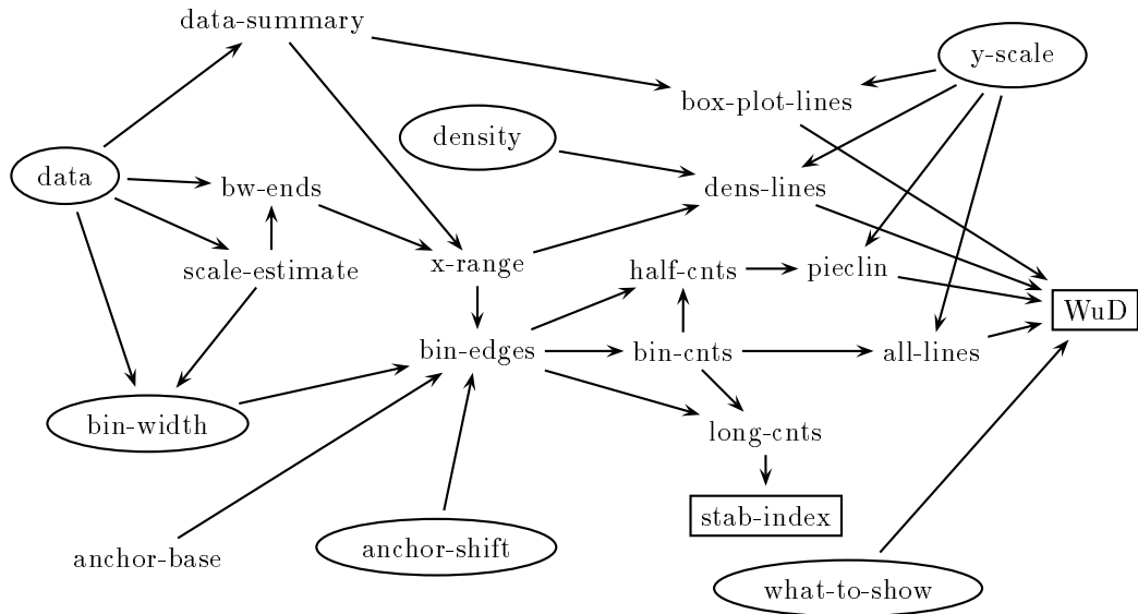
Figure 8: A directed graph to represent the flow of computation. Changes go forward, computation goes backward. Input quantities are shown in oval frames, the output ones in rectangular frames. WuD stands for the Window up to date flag.
