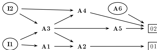
Figure 1: A directed graph to represent the flow of computation. Changes go forward, computation goes backward.
