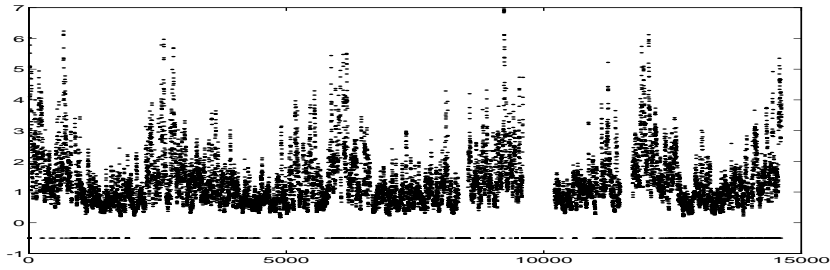
Figure 1: Significant wave height series and the missing data in the lower line.
