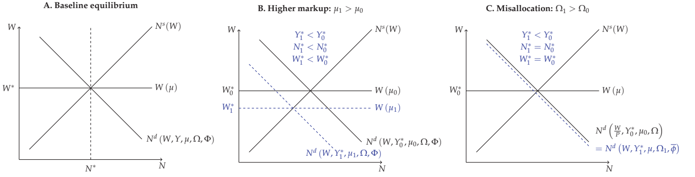
Figure 1: General equilibrium
