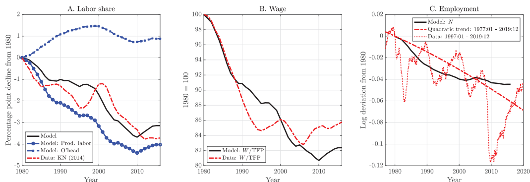
Figure 5: Aggregates
