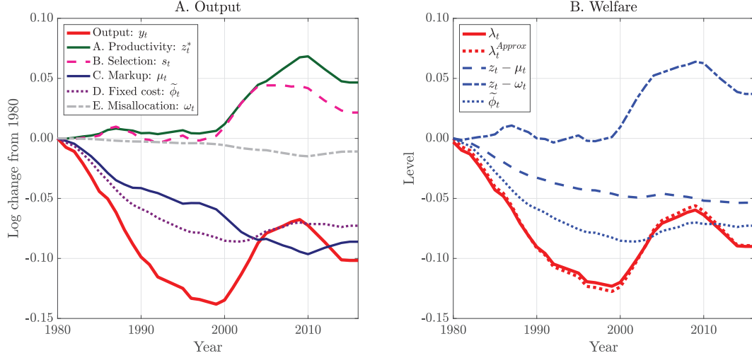
Figure 10: Decomposing output
