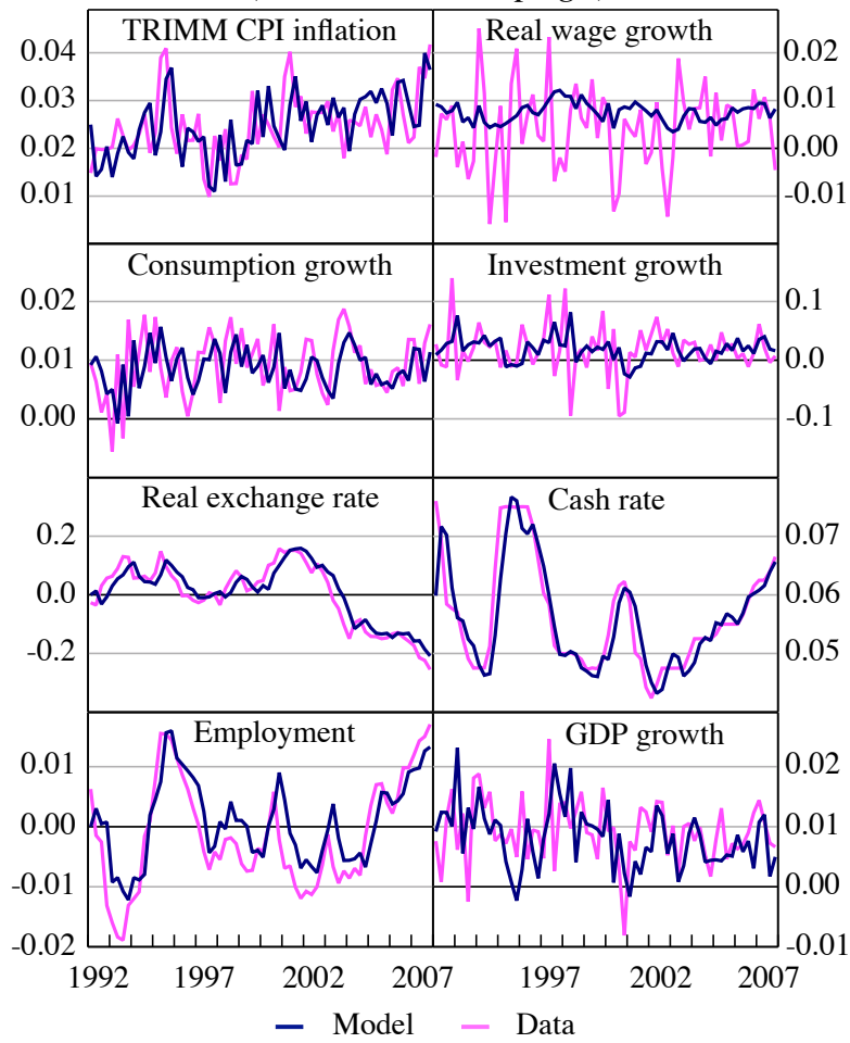
Figure 1: One-sided Fitted Values
